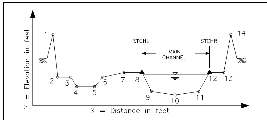
Figure A1-4 Example of Method 1 Encroachment to Keep Flow in the Main
